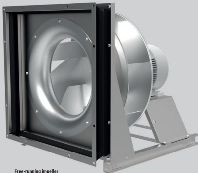
Free-running impeller For use in air handling units
